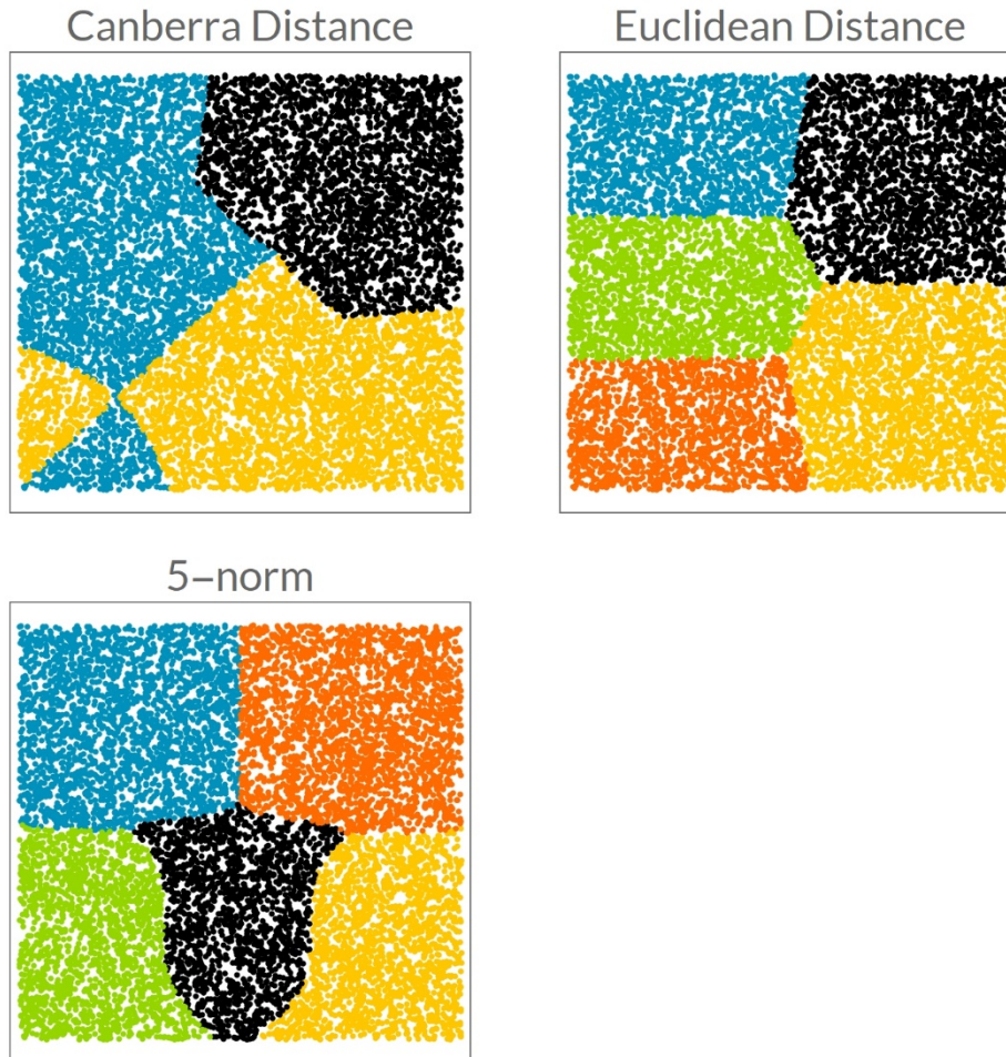
Figure 6: Clusters that depend on the choice of the distance function
