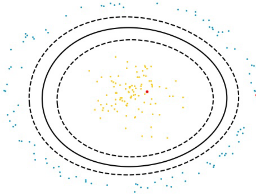
Figure 4: Polynomial SVM frontier separating two clusters of points
